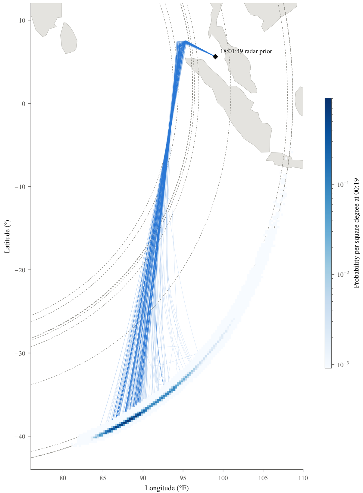
Figure 2. Posterior aircraft position at 00:19 UTC with BTO and BFO, pooled over 8 replicates (blue shading, logarithmic), and 400 routes drawn in proportion to posterior weight from replicate seed 1 (thin lines, 10-minute vertices). Dashed grey curves are the BTO arcs at a reference altitude of 35,000 ft; they are drawn for orientation only. Land: Natural Earth 1:110m.
